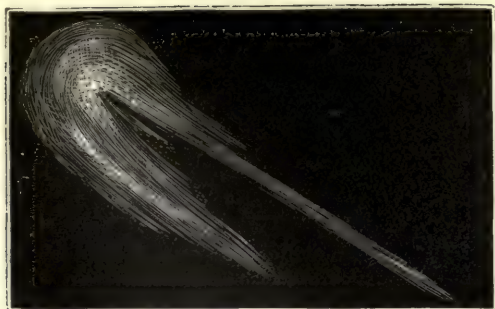
July 8. (Webb.)
